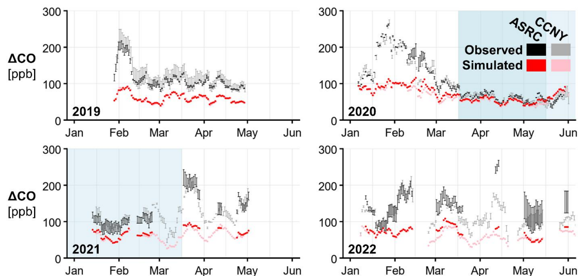
280 Figure 2. Timeseries of 10-day mean observed (black/grey) and simulated (red/pink) \Delta\text{CO} for the New York City Metropolitan Area (NYCMA) domain at the ASRC (black/red) and CCNY (grey/pink) sites during January–May 2019–2022. The observed \Delta\text{CO} vertical range represents the uncertainty in the background CO. \Delta\text{CO} are plotted at the center of the 10-day averaging period. The COVID-19 shutdown periods are shaded in blue: peak (darker, 15 March–15 May 2020) and residual (lighter, 16 May 2020–15 March 2021).
