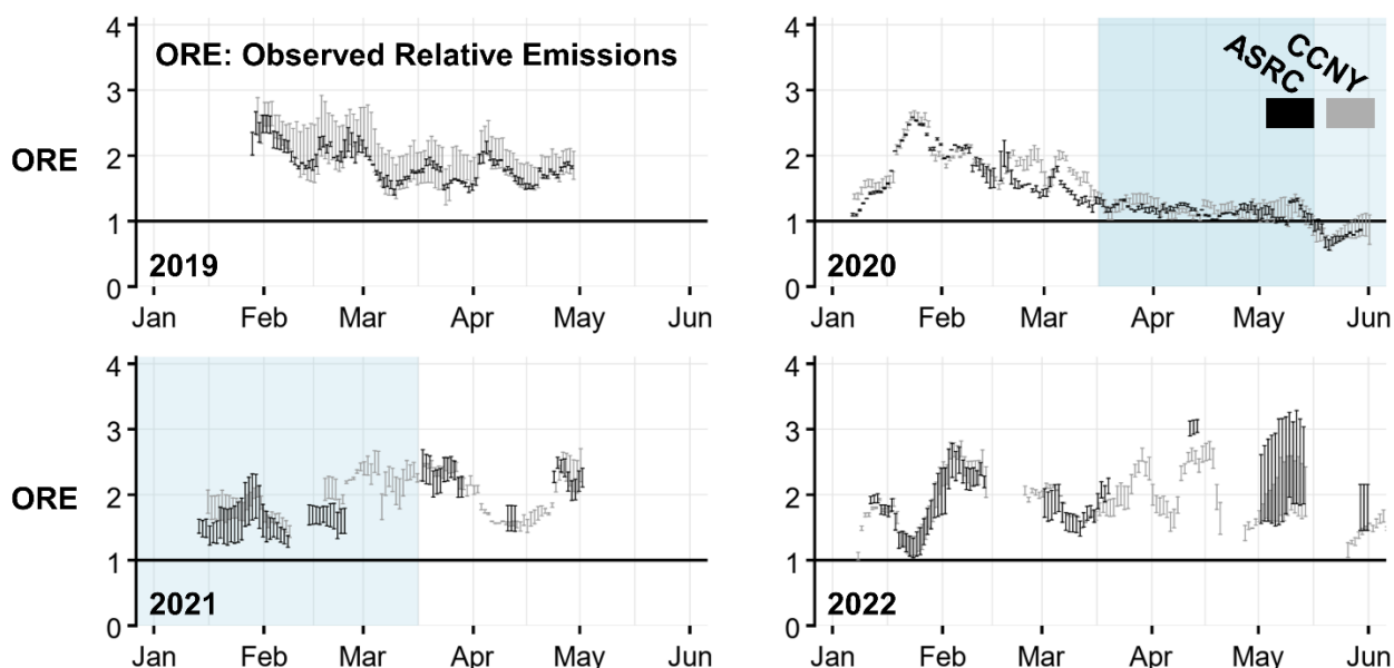
Figure 5. Timeseries of observed relative emissions (ORE) for the NYCMA domain at the ASRC (black) and CCNY (grey) sites during January–May 2019–2022, where ORE is the ratio of observed \Delta\text{CO} to simulated \Delta\text{CO} using EDGAR from Fig. 2. The vertical range represents the uncertainty in the background CO. ORE is plotted at the center of the 10-day averaging period. The COVID-19 shutdown periods are shaded in blue: peak (darker, 15 March–15 May 2020) and residual (lighter, 16 May 2020–15 March 2021).
